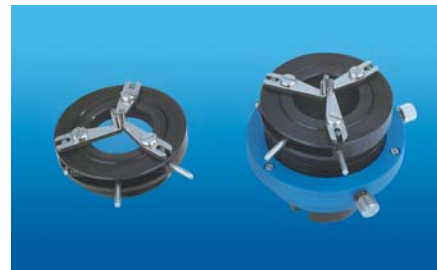
Self-centering mount 3-35mm with X,Y-translation capabilities
