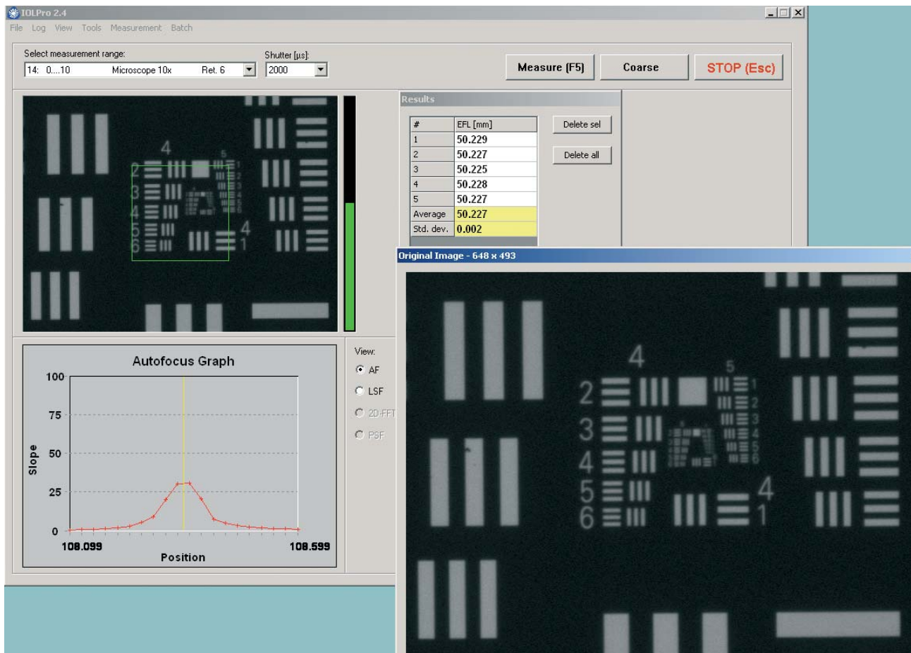
IOL Measurement –EFL, MTF, Resolution Efficiency
